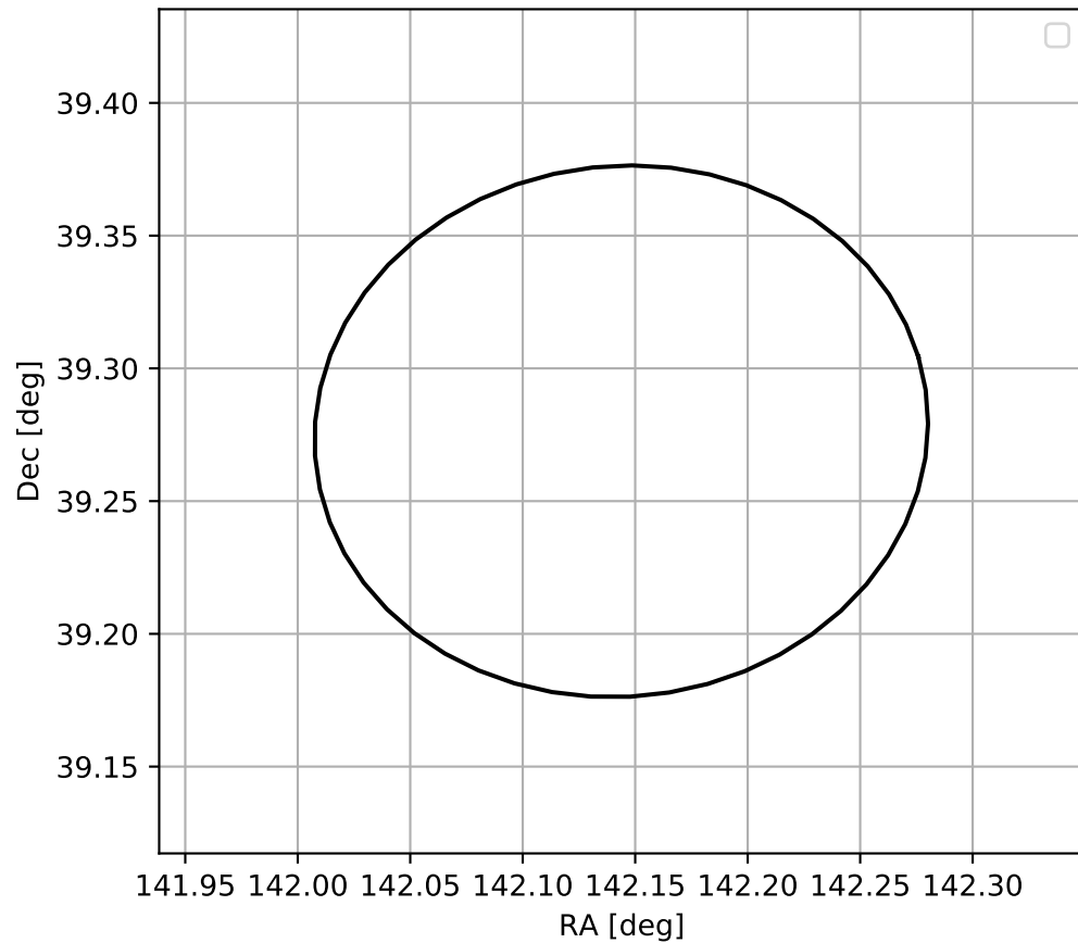
4FGL J0928.5+3916
