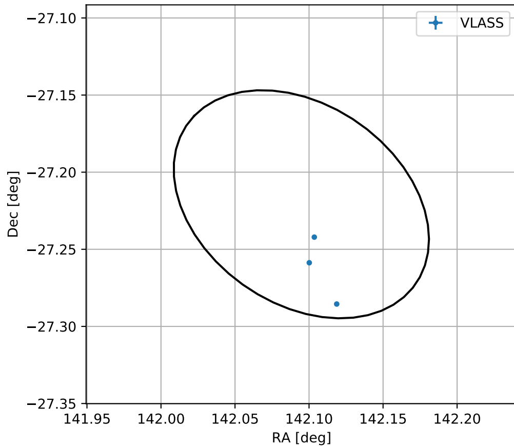
4FGL J0928.3-2713
