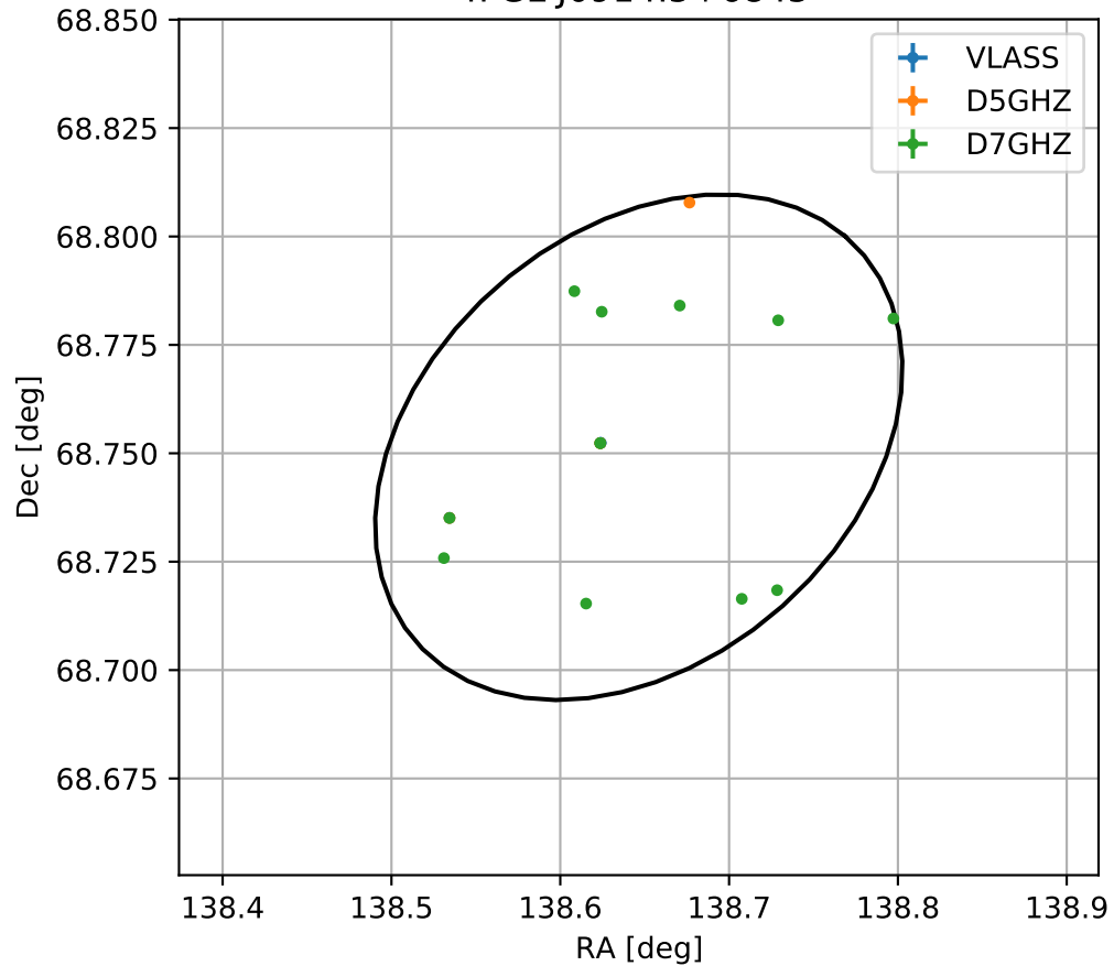
4FGL J0914.5+6845
