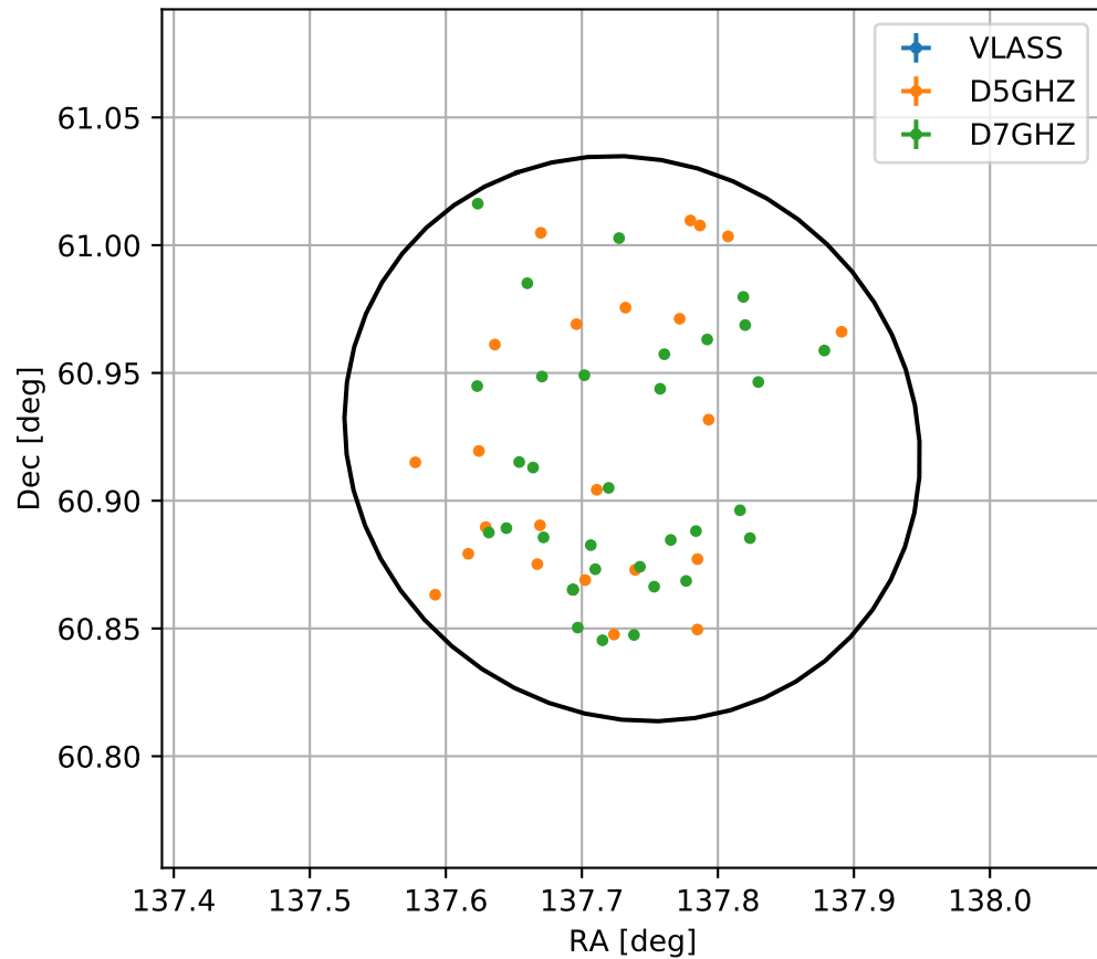
4FGL J0910.9+6055
