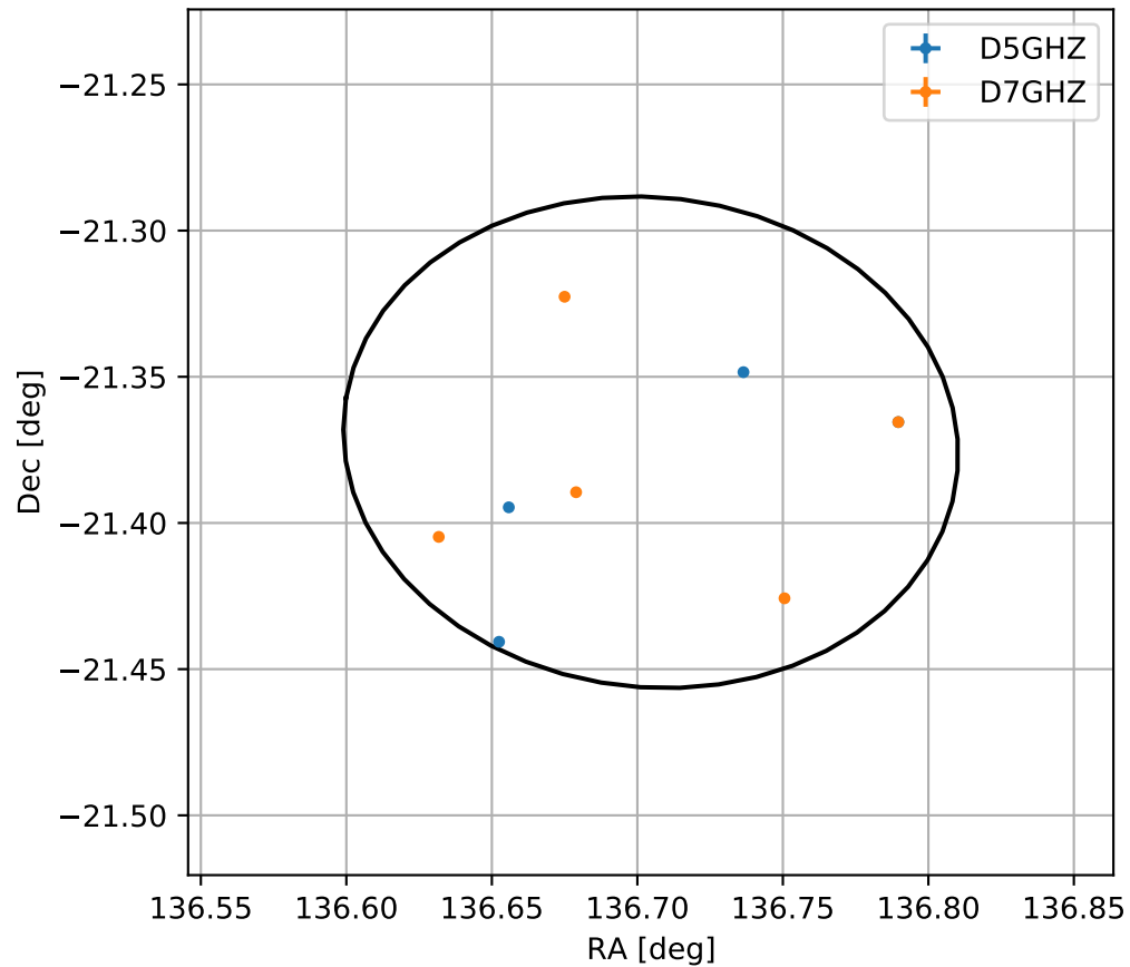
4FGL J0906.8-2122
