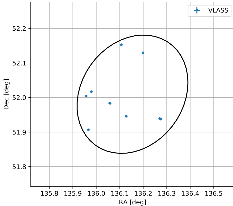
4FGL J0904.6+5200
