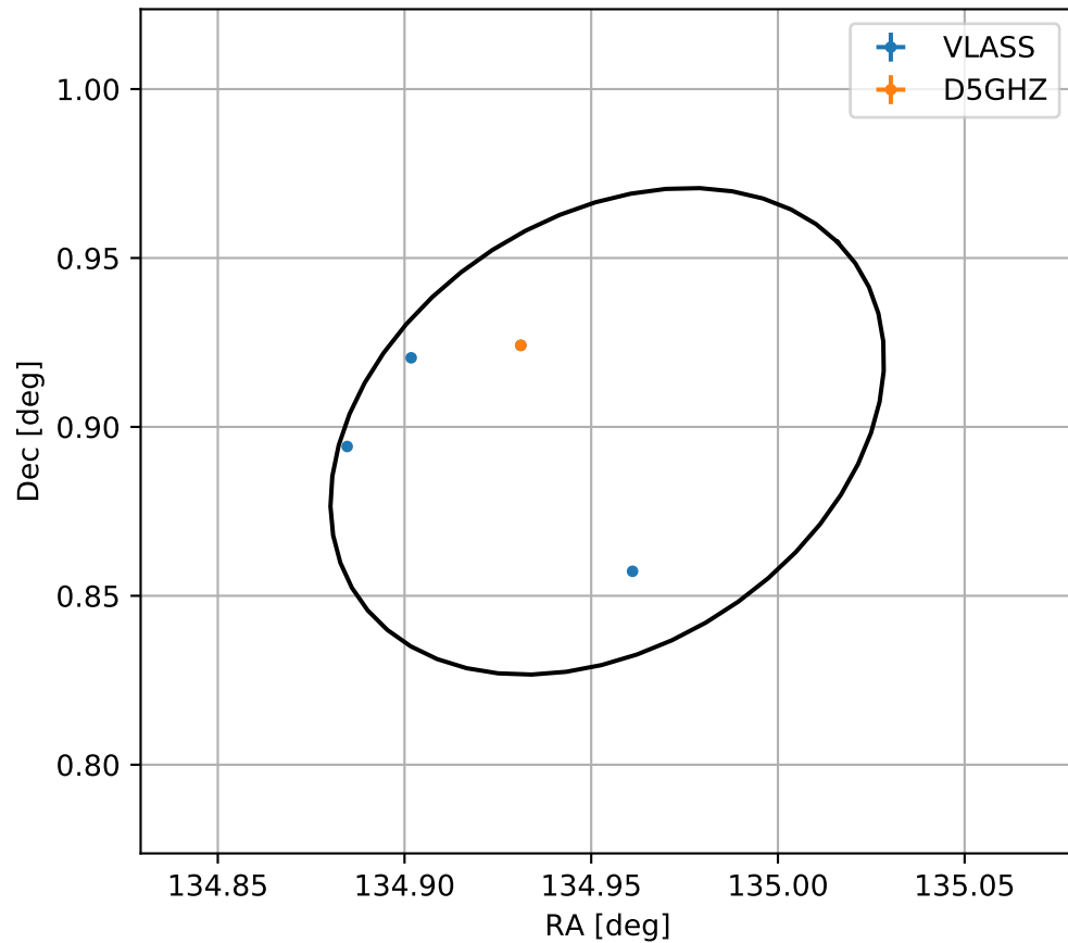
4FGL J0859.8+0053
