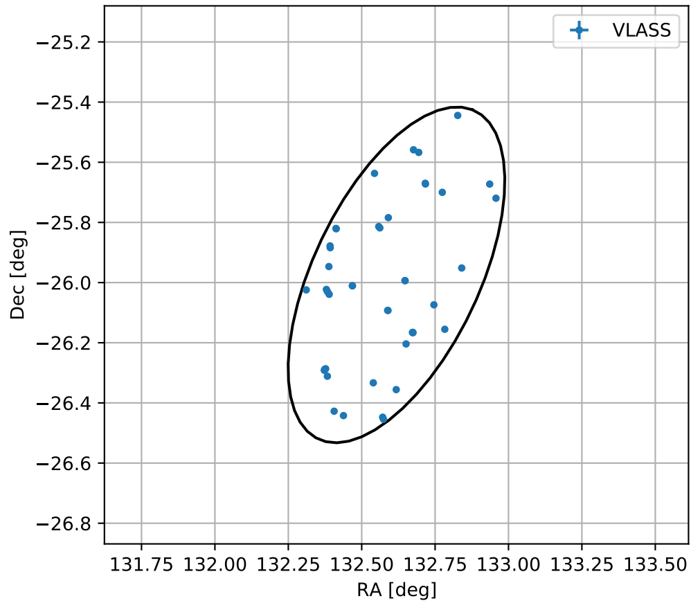
4FGL J0850.4-2558
