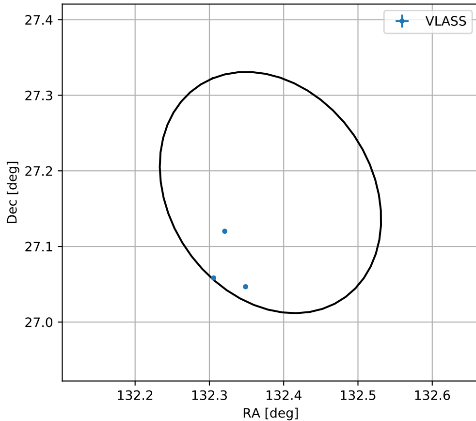
4FGL J0849.5+2710
