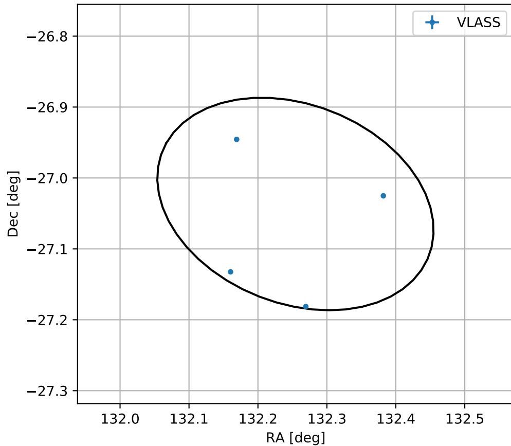
4FGL J0849.0-2702
