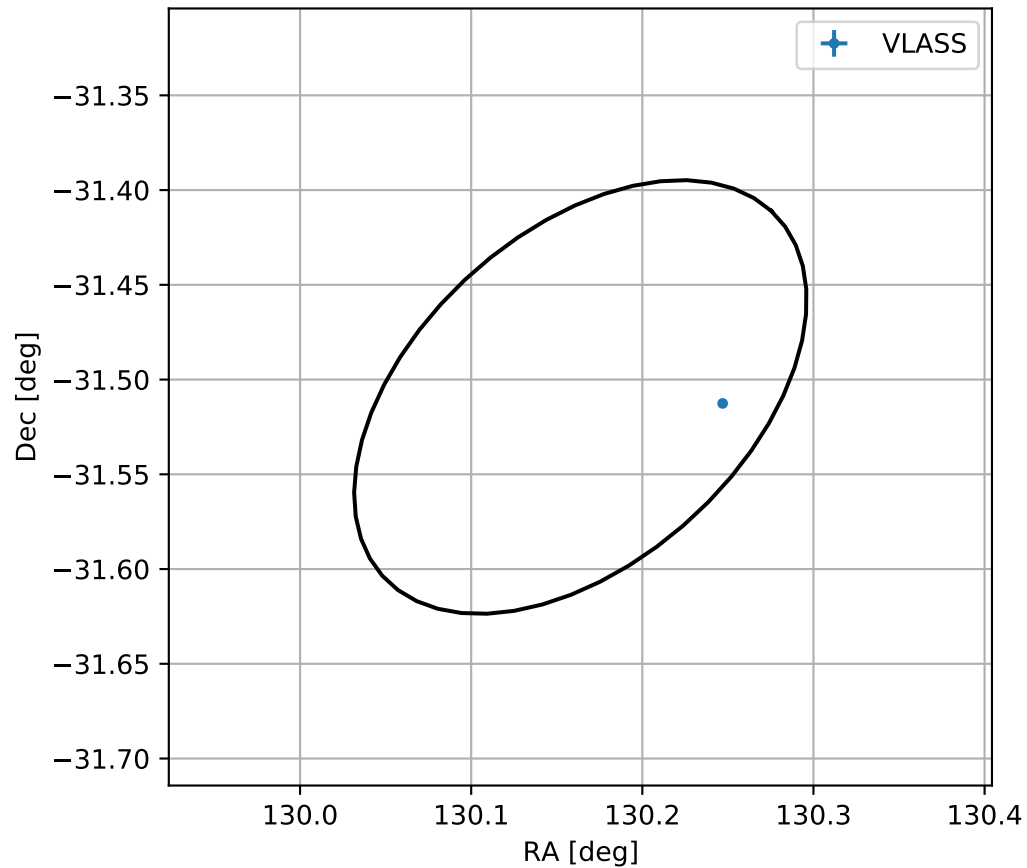
4FGL J0840.6-3130
