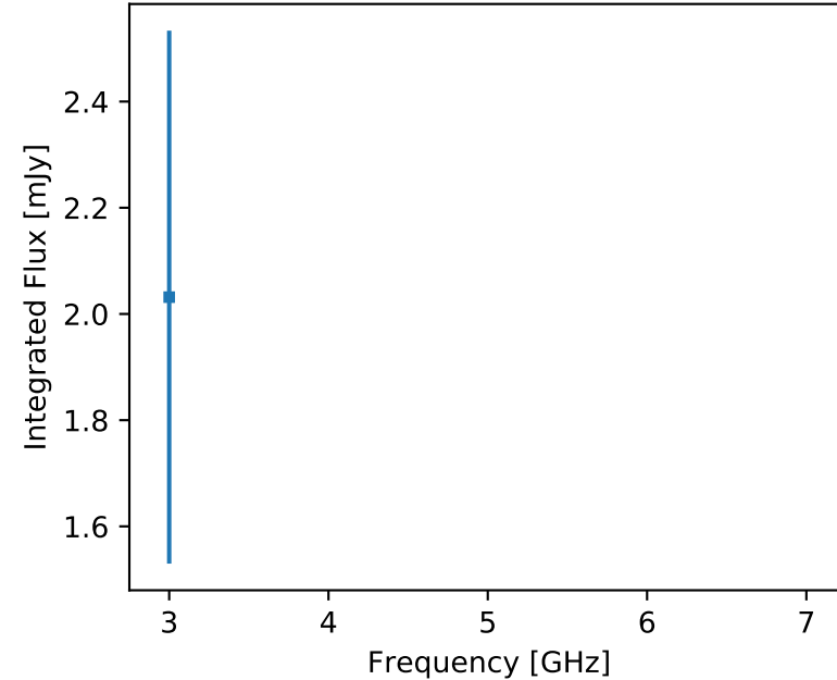
F357 J084059.26-313045.3 (unr)
