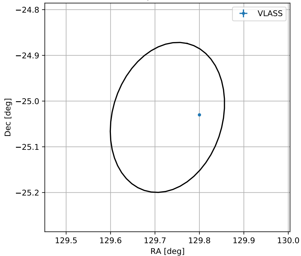
4FGL J0838.9-2502
