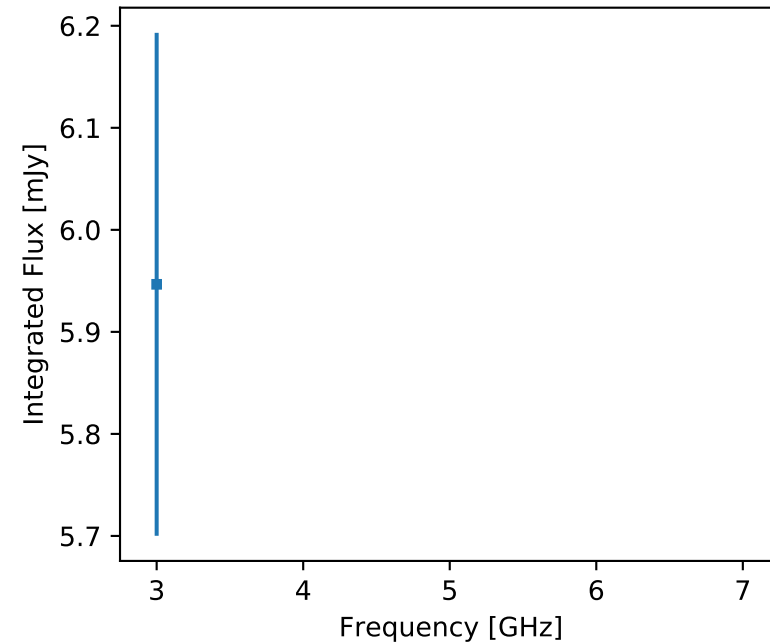
F357 J083912.02-250148.4 (unr)
