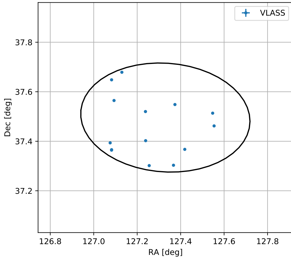
4FGL J0829.3+3729
