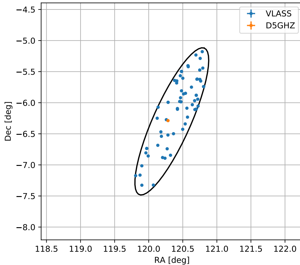
4FGL J0801.3-0617
