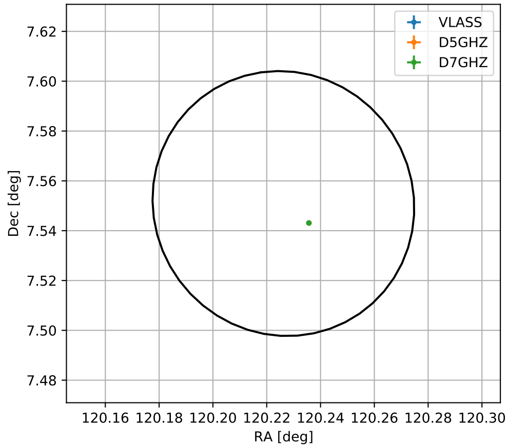
4FGL J0800.9+0733
