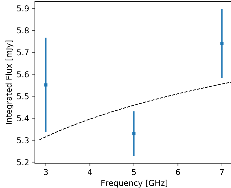
F357 J080056.56+073235.1 (unr)
