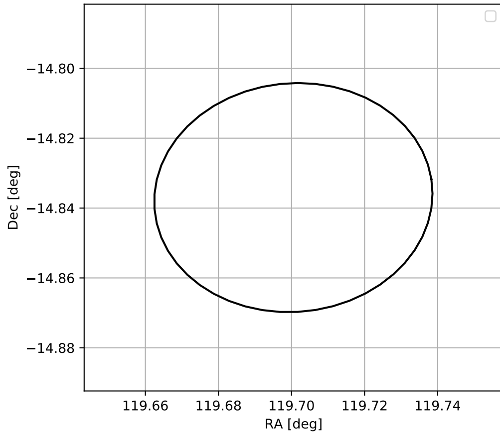
4FGL J0758.8-1450
