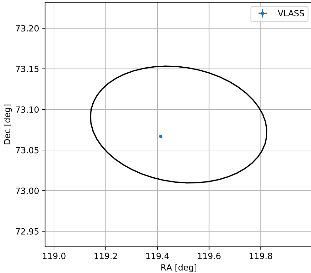
4FGL J0757.9+7304
