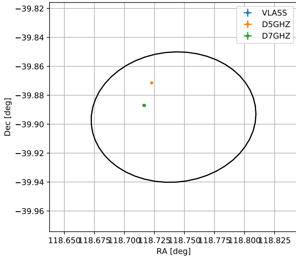
4FGL J0754.9-3953
