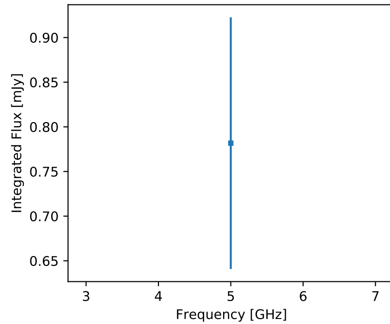
F357 J075453.44-395217.1 (unr)
