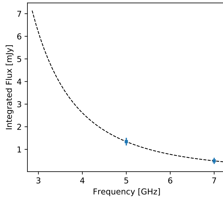
F357 J075452.00-395313.3 (unr)
