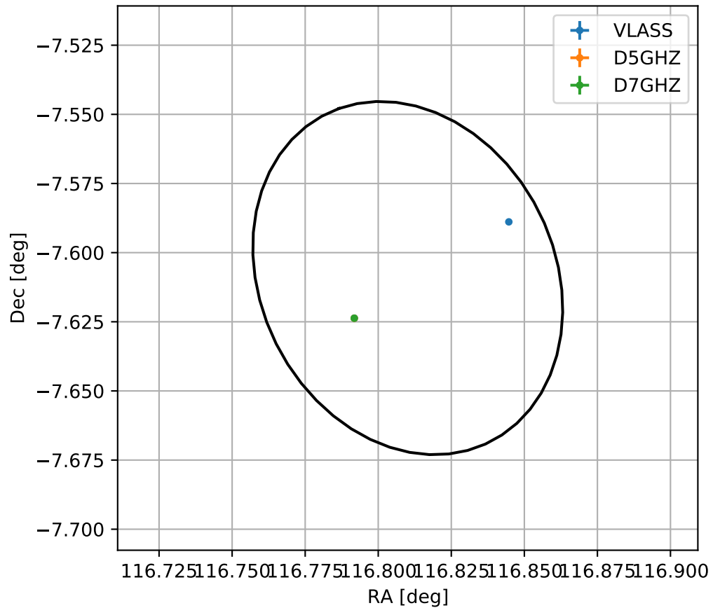
4FGL J0747.2-0736
