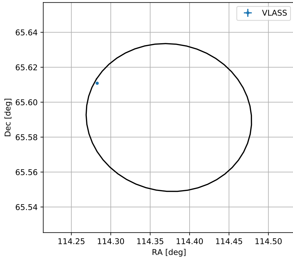
4FGL J0737.4+6535
