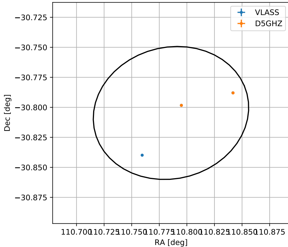
4FGL J0723.1-3048
