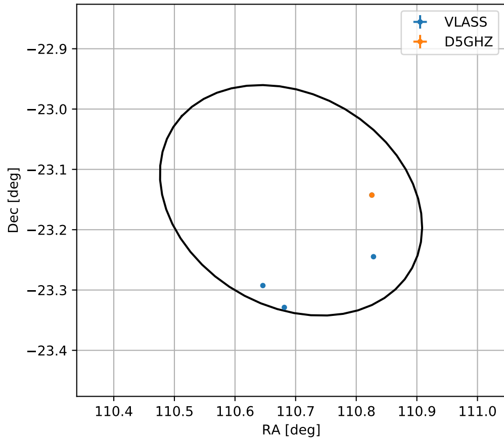
4FGL J0722.7-2309c
