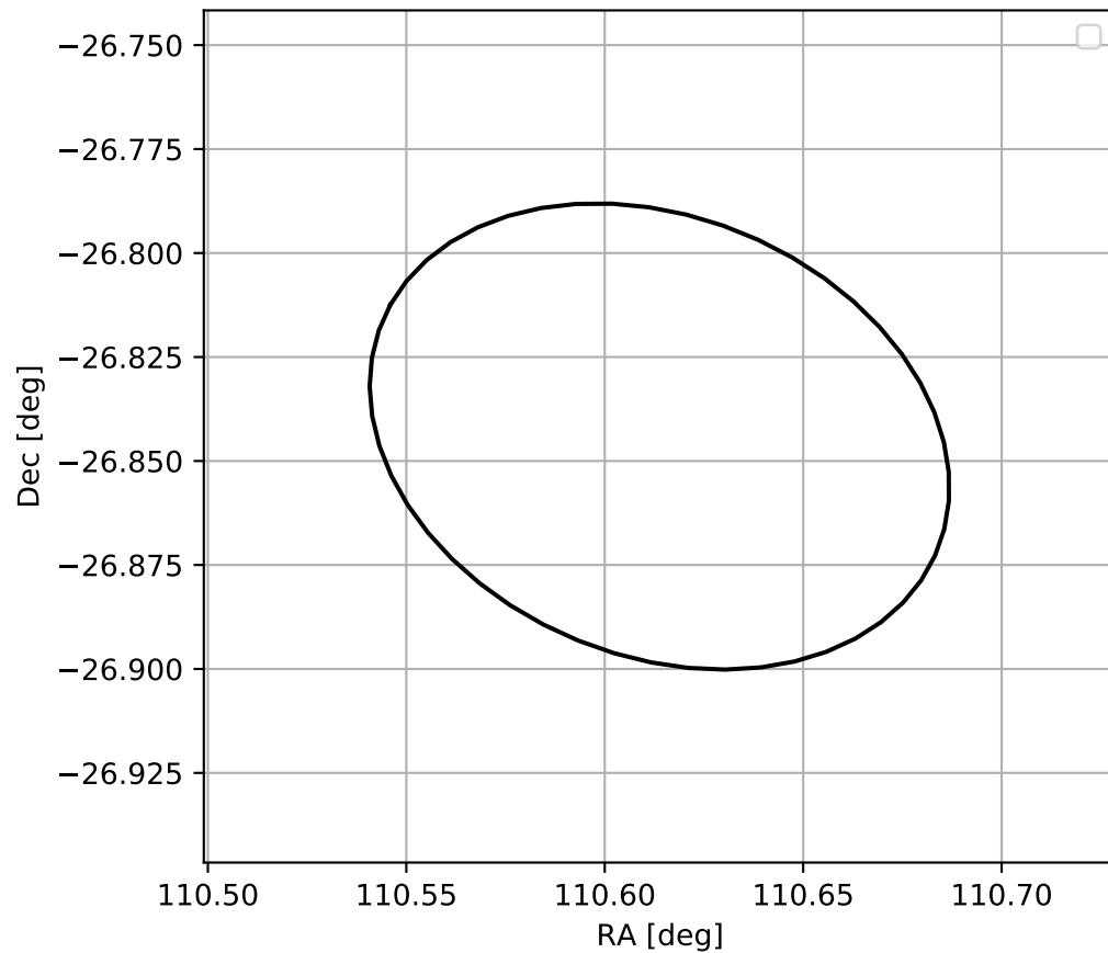
4FGL J0722.4-2650
