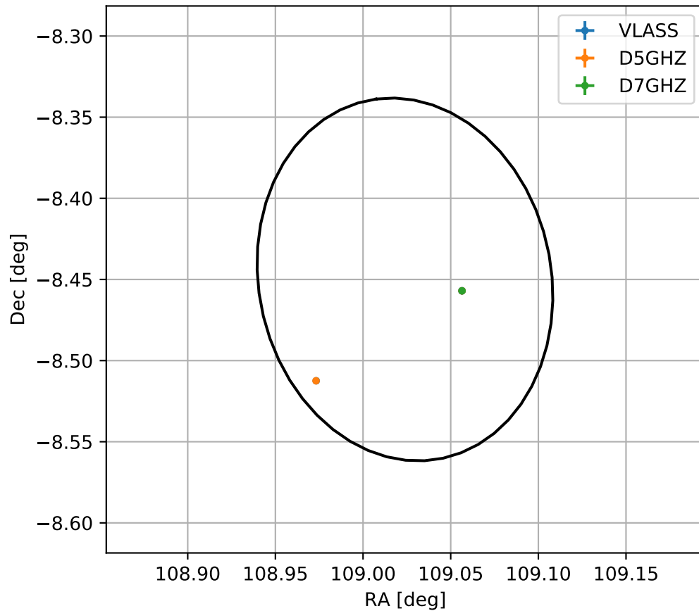
4FGL J0716.0-0826
