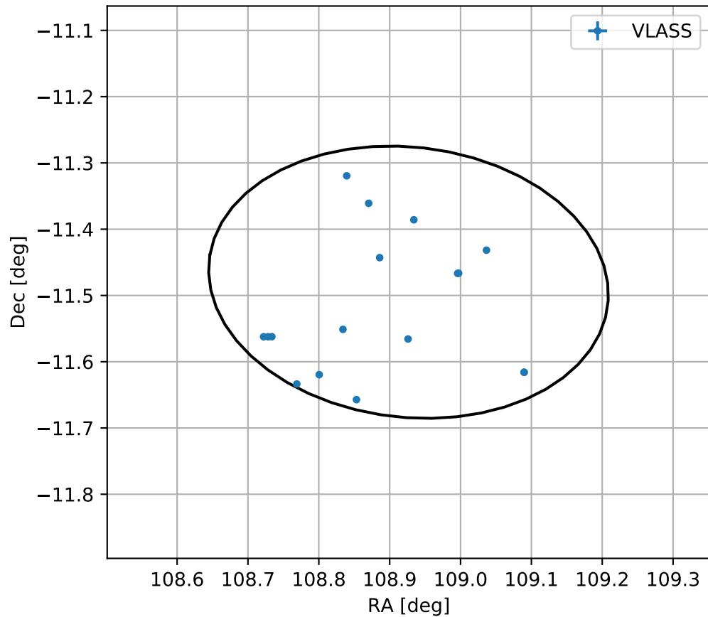
4FGL J0715.7-1128
