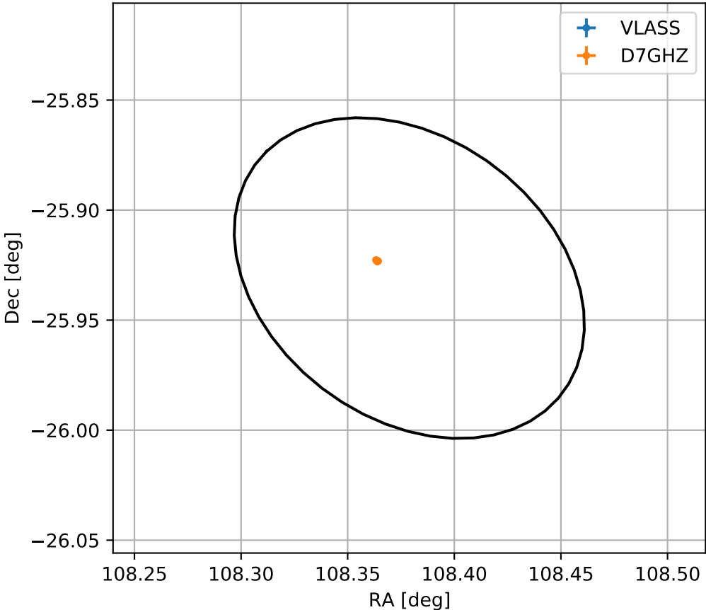
4FGL J0713.5-2555
