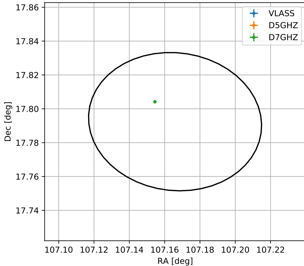
4FGL J0708.6+1747
