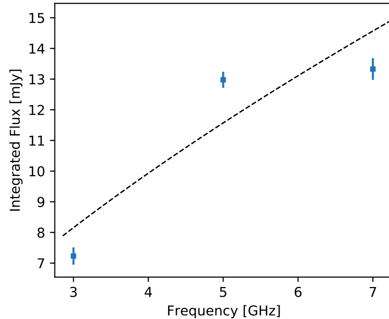
F357 J070837.07+174814.8 (res)
