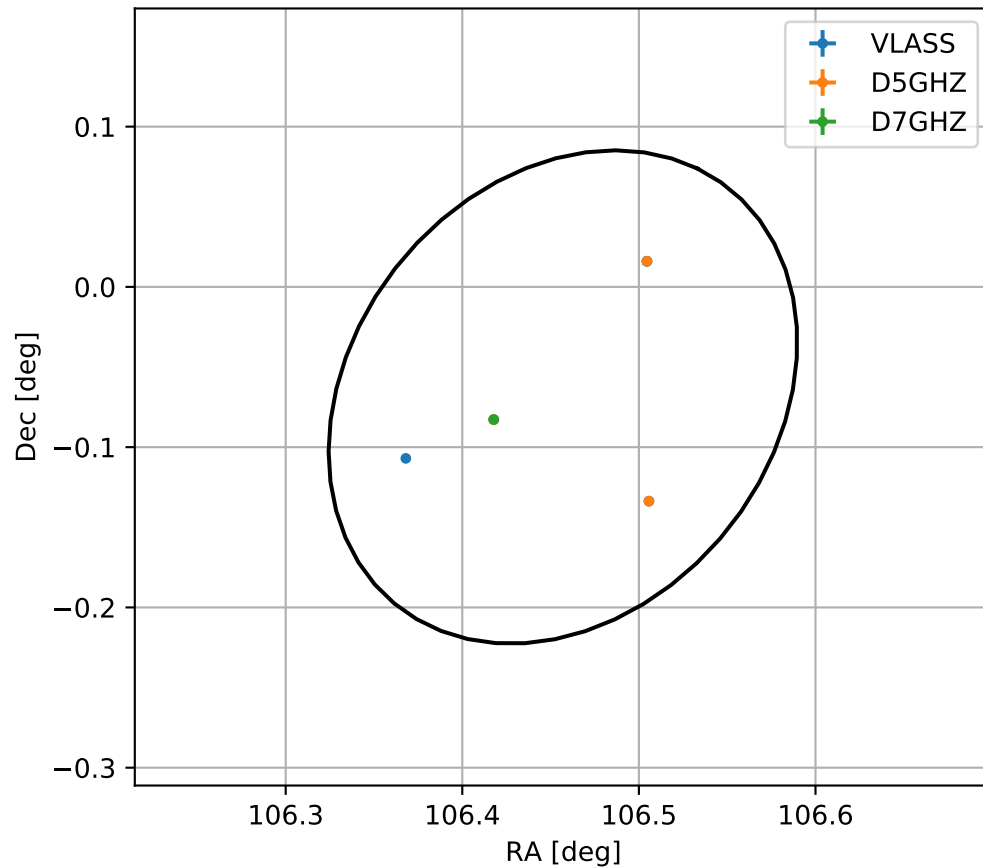
4FGL J0705.8-0004
