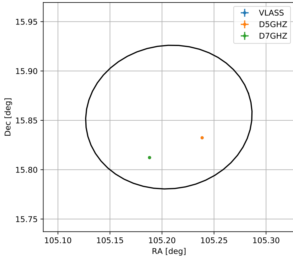
4FGL J0700.8+1551
