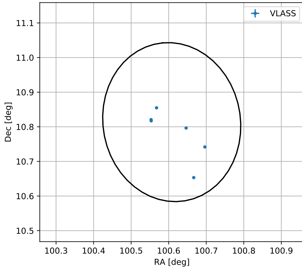
4FGL J0642.4+1048
