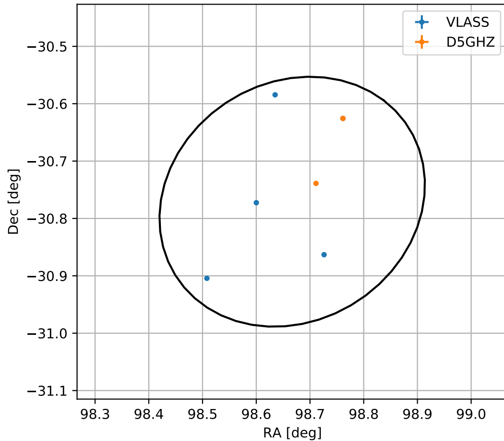
4FGL J0634.6-3046c
