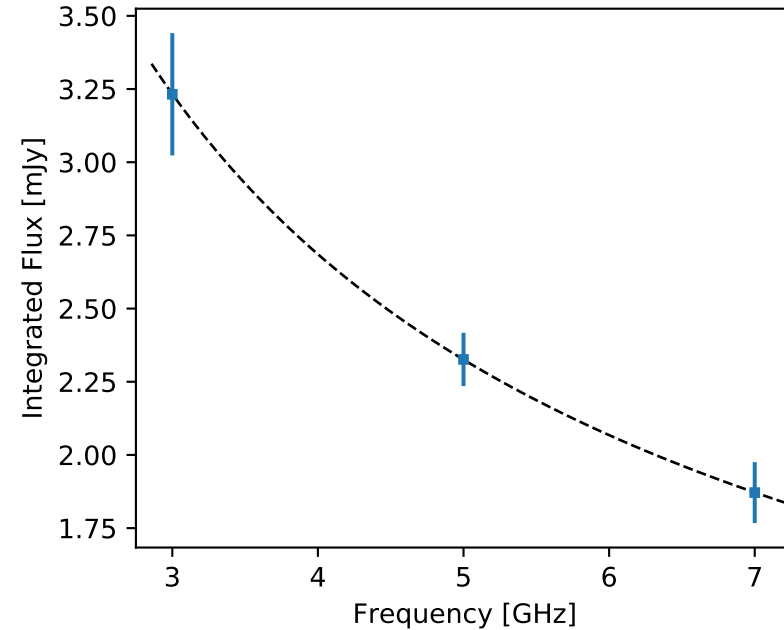
F357 J062535.58+702940.7 (unr)
