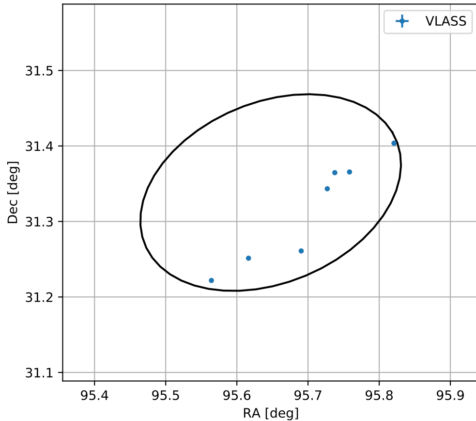
4FGL J0622.5+3120
