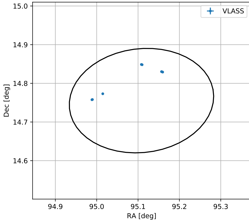
4FGL J0620.4+1445
