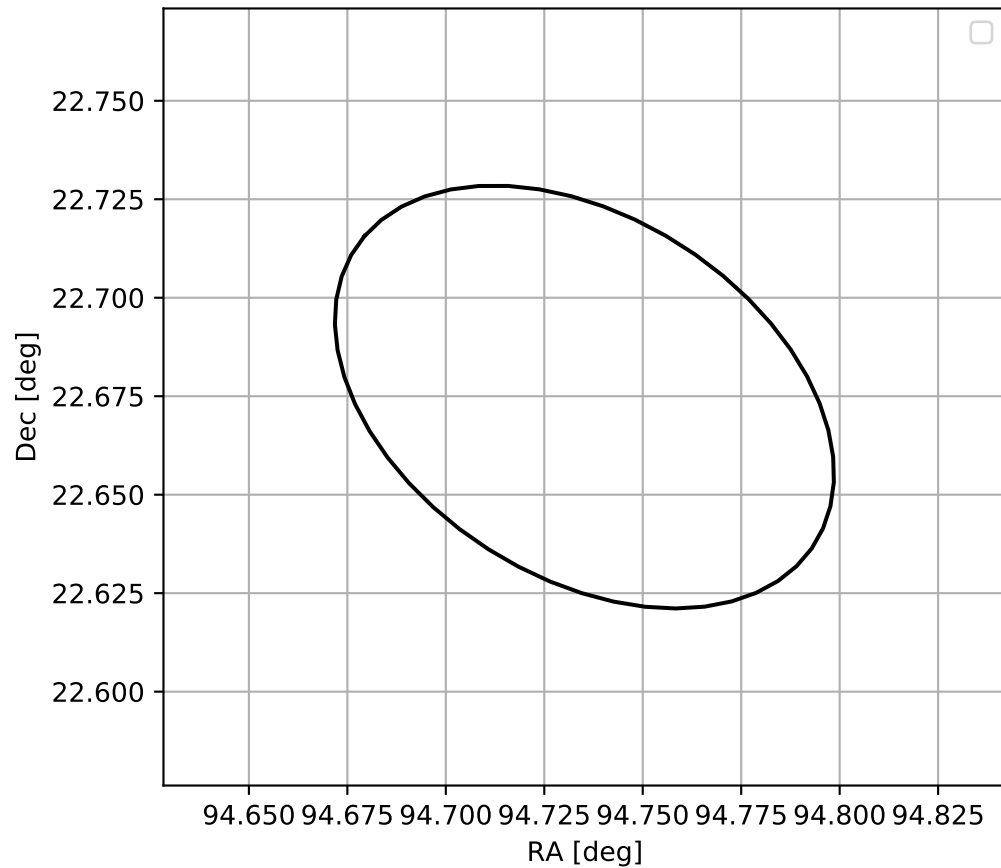
4FGL J0618.9+2240c
