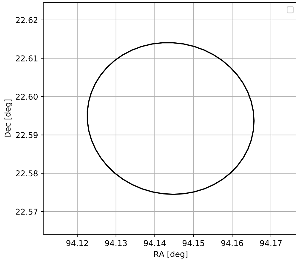
4FGL J0616.5+2235
