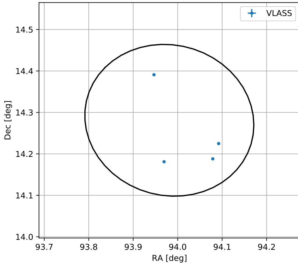
4FGL J0615.9+1416
