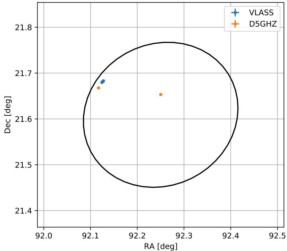
4FGL J0609.0+2136c
