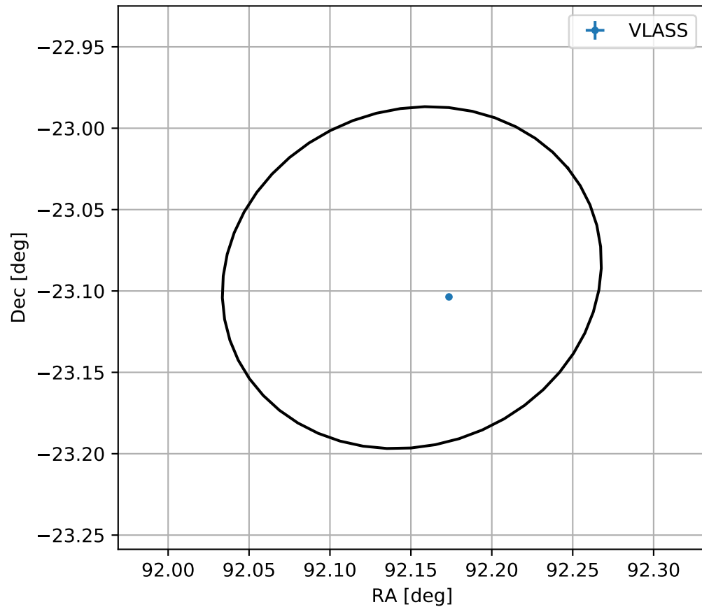
4FGL J0608.6-2305
