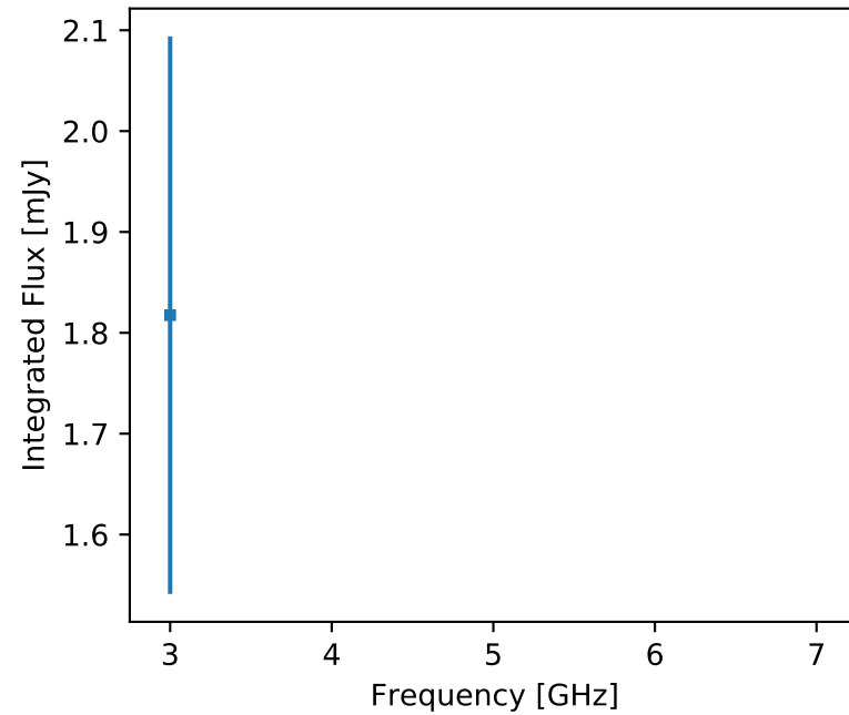
F357 J060802.28-190619.0 (unr)
