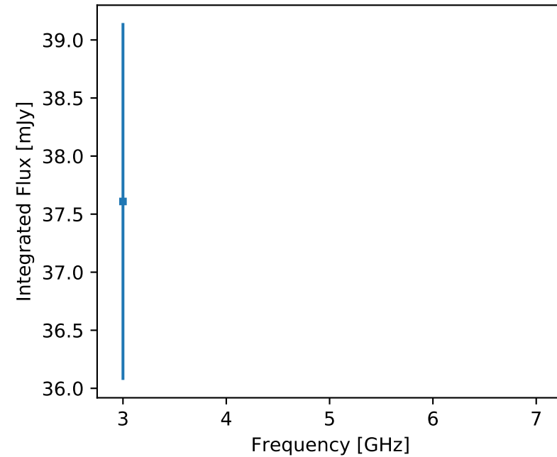
F357 J060802.28-190619.0 (unr)
