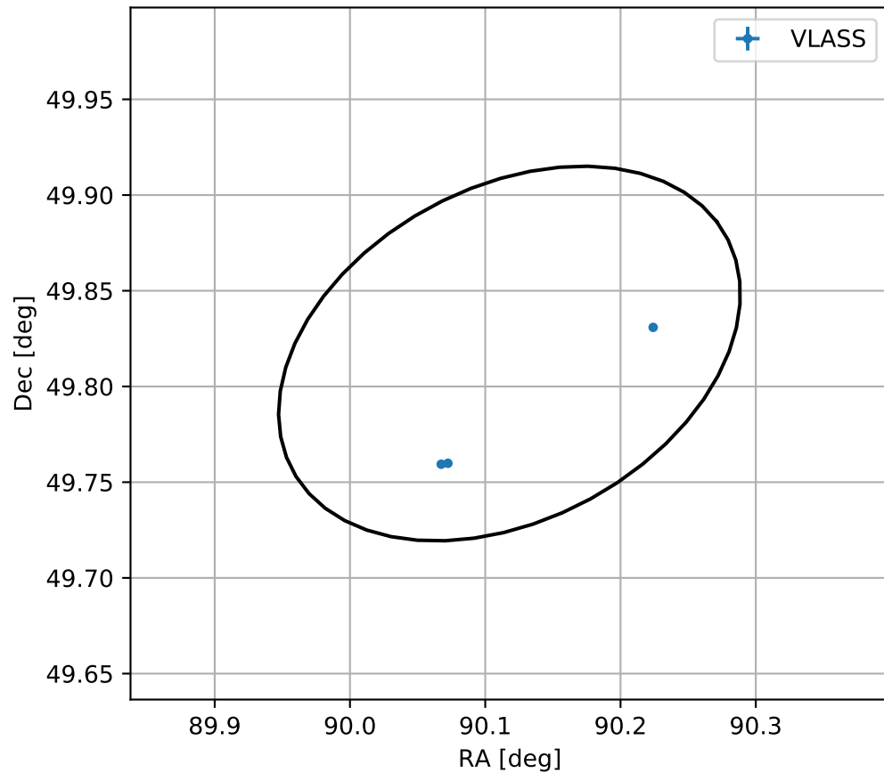
4FGL J0600.4+4949
