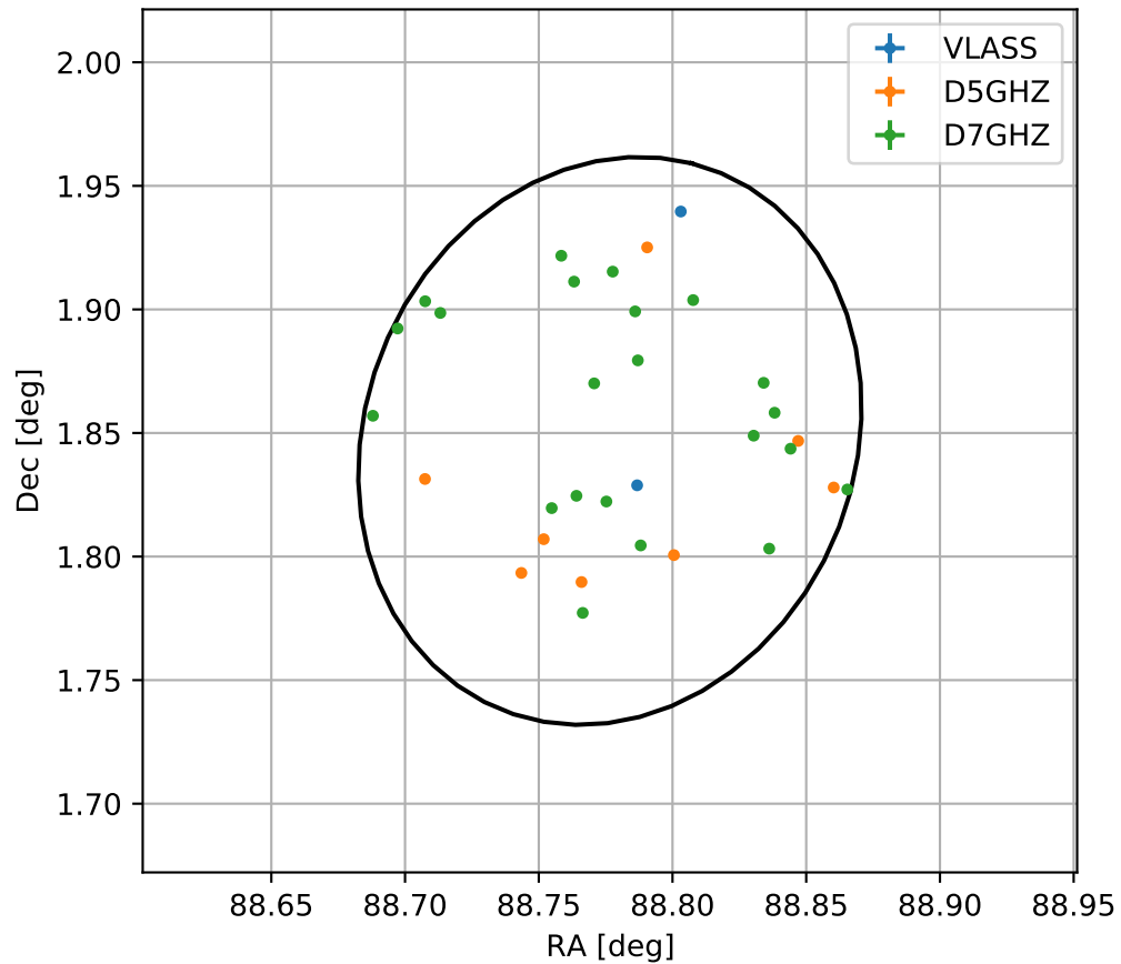
4FGL J0555.1+0150c
