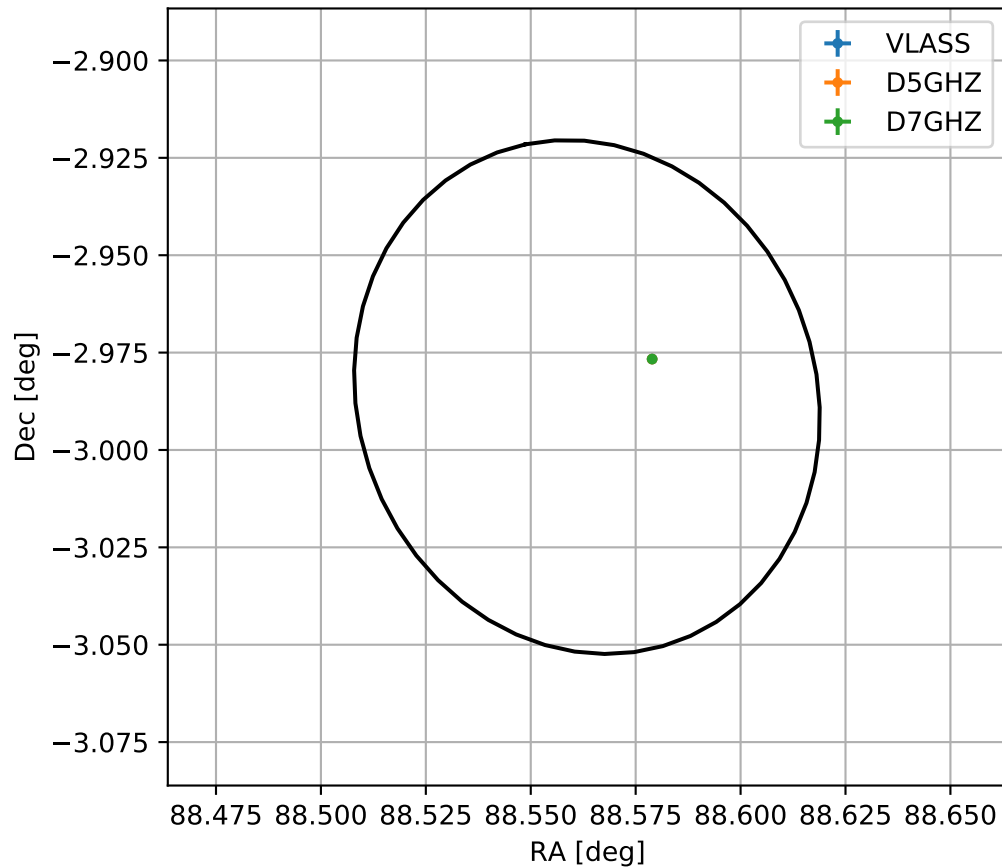
4FGL J0554.2-0259
