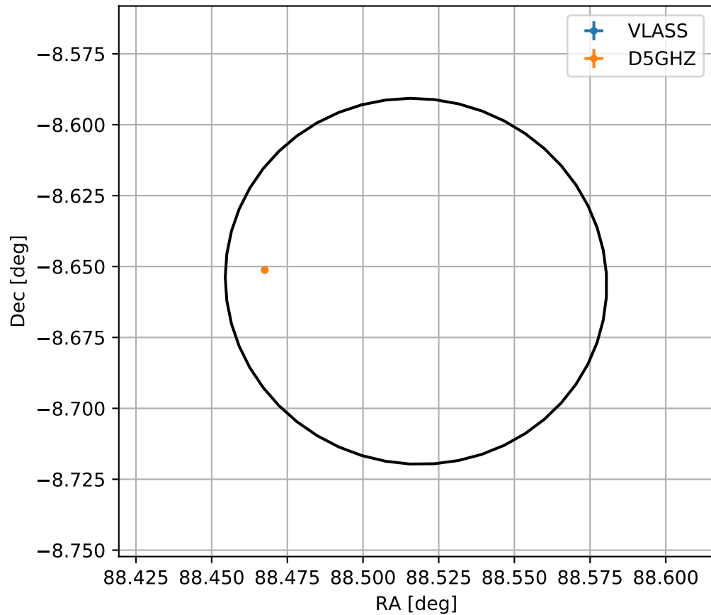
4FGL J0554.0-0839
