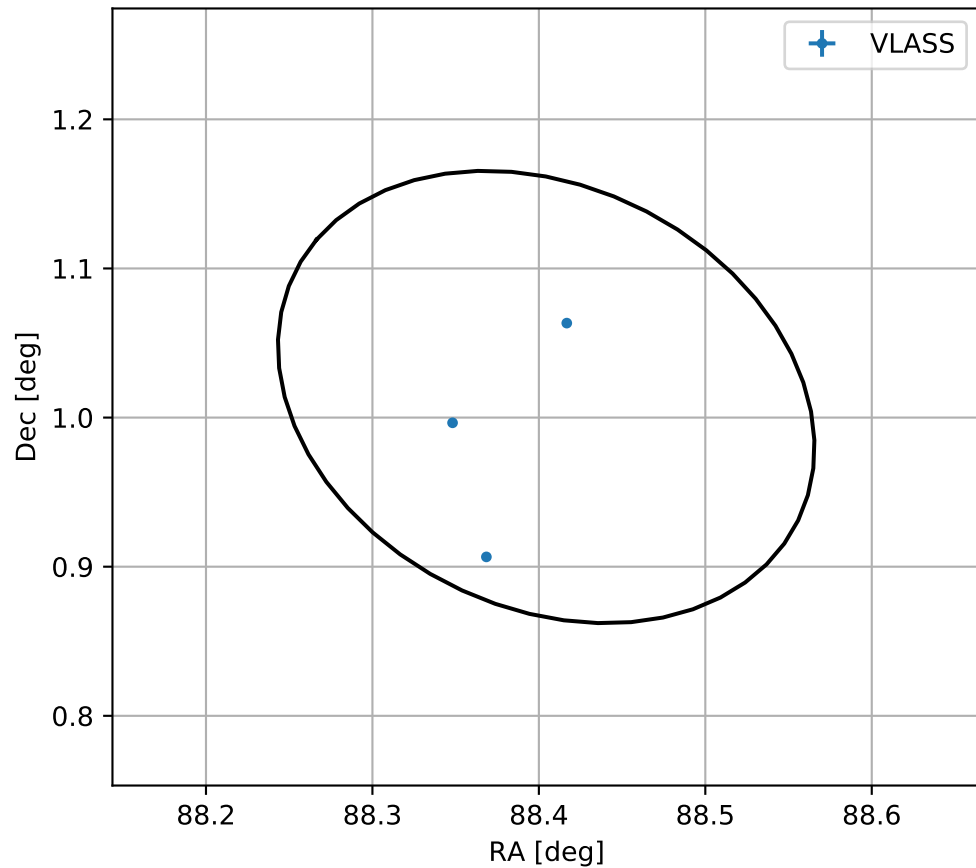
4FGL J0553.6+0100
